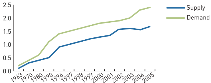
Fig A: Groundwater demand and supply in Dhaka City from 1963 to 2005
